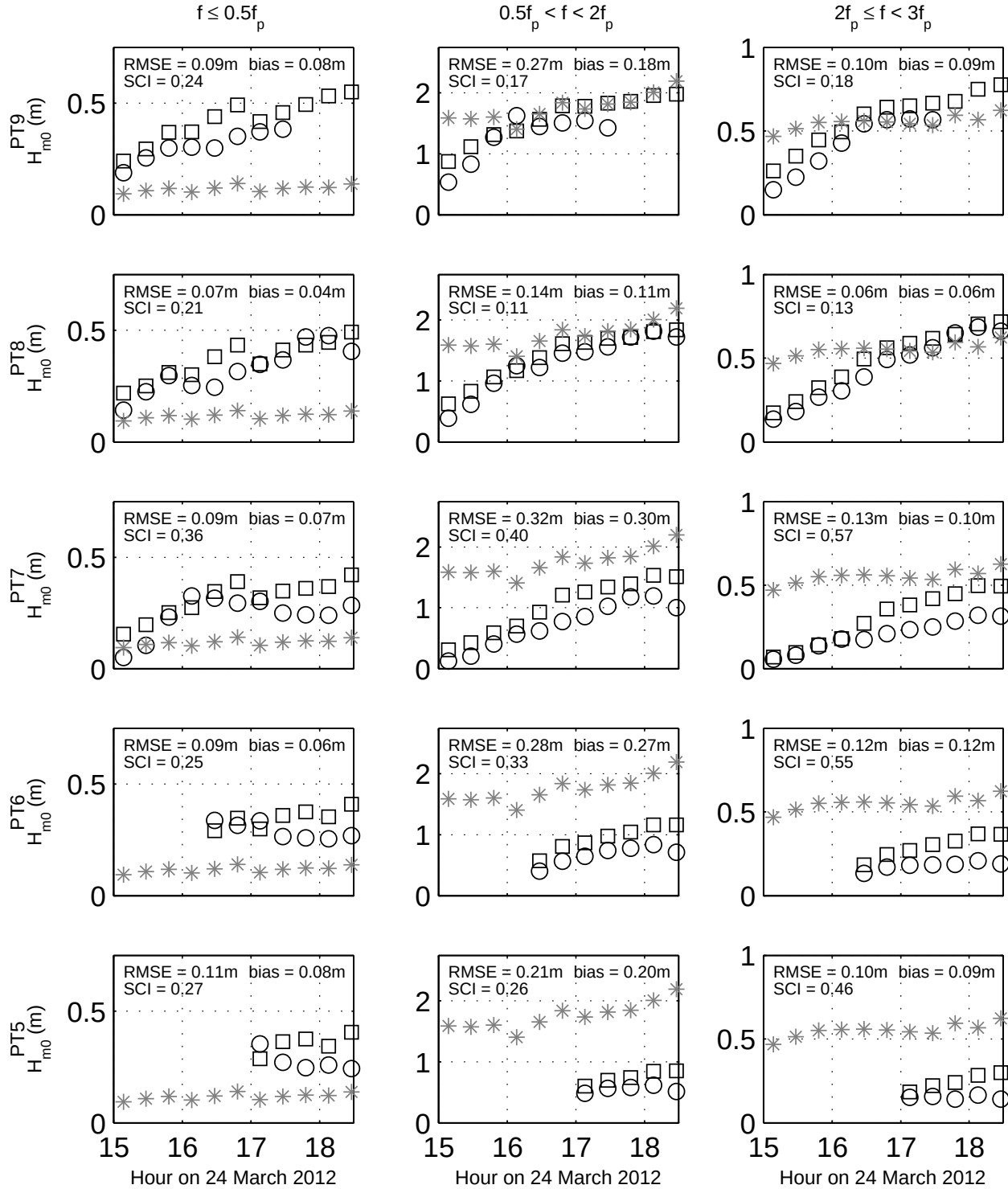
Figure 7: Significant offshore wave height time series (*), significant wave height time series measured by five nearshore pressure transducers (○) and significant wave height time series modelled at the location of the nearshore pressure transducers (□) during LB2, separated into three frequency bands, where f_p represents the offshore spectral peak frequency. The locations of the five nearshore pressure transducers in the cross-shore are shown in Figure 3.
