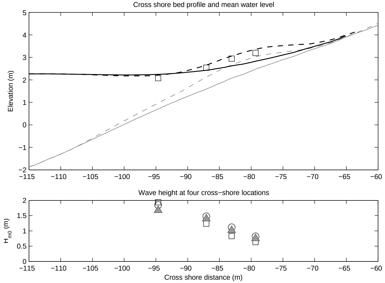
Figure 15: Effect of bed level updates on computed mean water levels and wave heights at Loe Bar. Top panel: measured 20-minute mean water at 18:00 during LB2(□), modelled mean water level without updated bed levels (black solid line) and modelled mean water level with updated bed levels (black dashed line). Bed levels corresponding to the period of the simulation without and with updated bed levels are indicated by the solid and dashed grey lines respectively. Bottom panel: measured wave height at 18:00 during LB2(□), modelled wave height without updated bed levels (○) and modelled wave height with updated bed levels (grey △).
